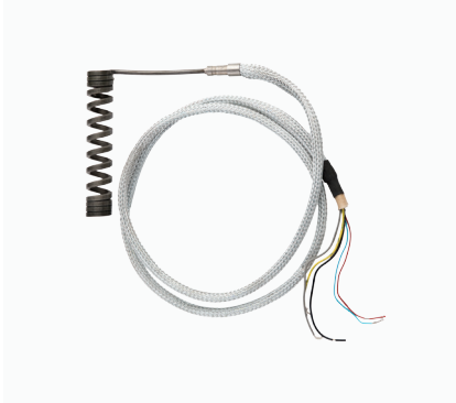
Coil Heater
